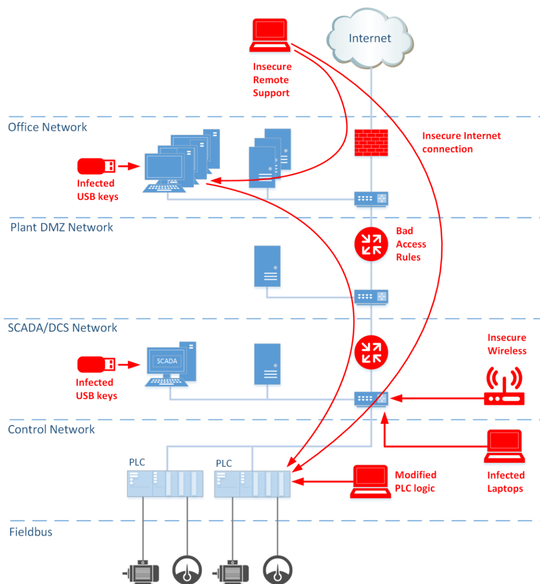
Cyberattack vectors
